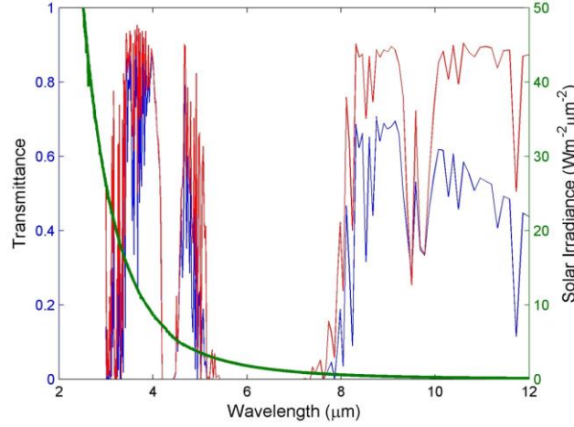
Figure 1. Simulated atmospheric transmittance for a US Standard Atmosphere (red) and tropical atmosphere (blue) in the 3–12 \mu\text{m} region. Also shown is the solar irradiance contribution \text{W}/\text{m}^2/\mu\text{m}^2 .
