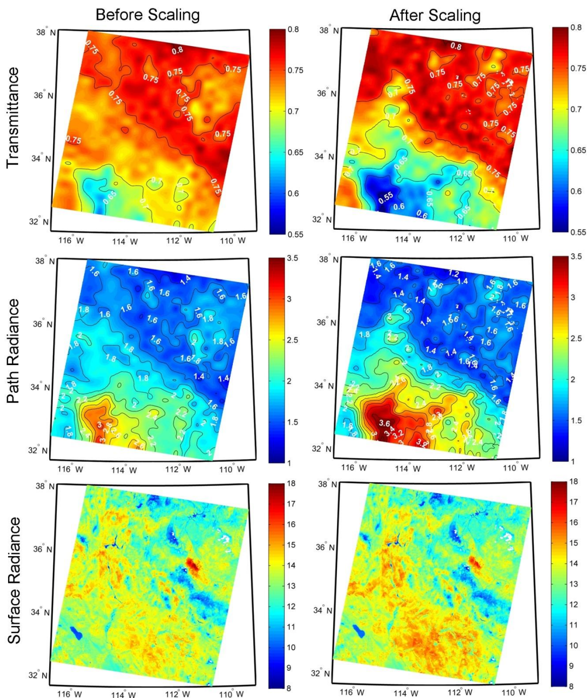
Figure 6. Comparisons between the atmospheric transmittance (top), path radiance ( \text{W}/\text{m}^2/\mu\text{m}^{-1} ) (middle), and computed surface radiance ( \text{W}/\text{m}^2/\mu\text{m}^{-1} ) (bottom), before and after applying the WVS scaling factor \gamma to a MODIS scene cutout shown in Figure 5. Results are shown for MODIS band 29 (8.55 \mu\text{m} ).
