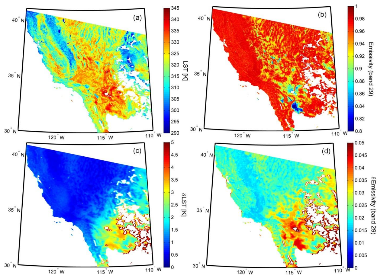
Figure 22. MODIS TES retrievals including WVS correction over the southwestern United States on 7 August 2004: (a) (top left) LST, (b) (top right) emissivity for band 29 (8.55 \mu\text{m} ), (c) (bottom left) LST uncertainty, and (d) (bottom right) emissivity uncertainty for band 29 (8.55 \mu\text{m} ). White areas over land indicate areas of cloud that have been masked out using the MOD35 cloud mask product.
