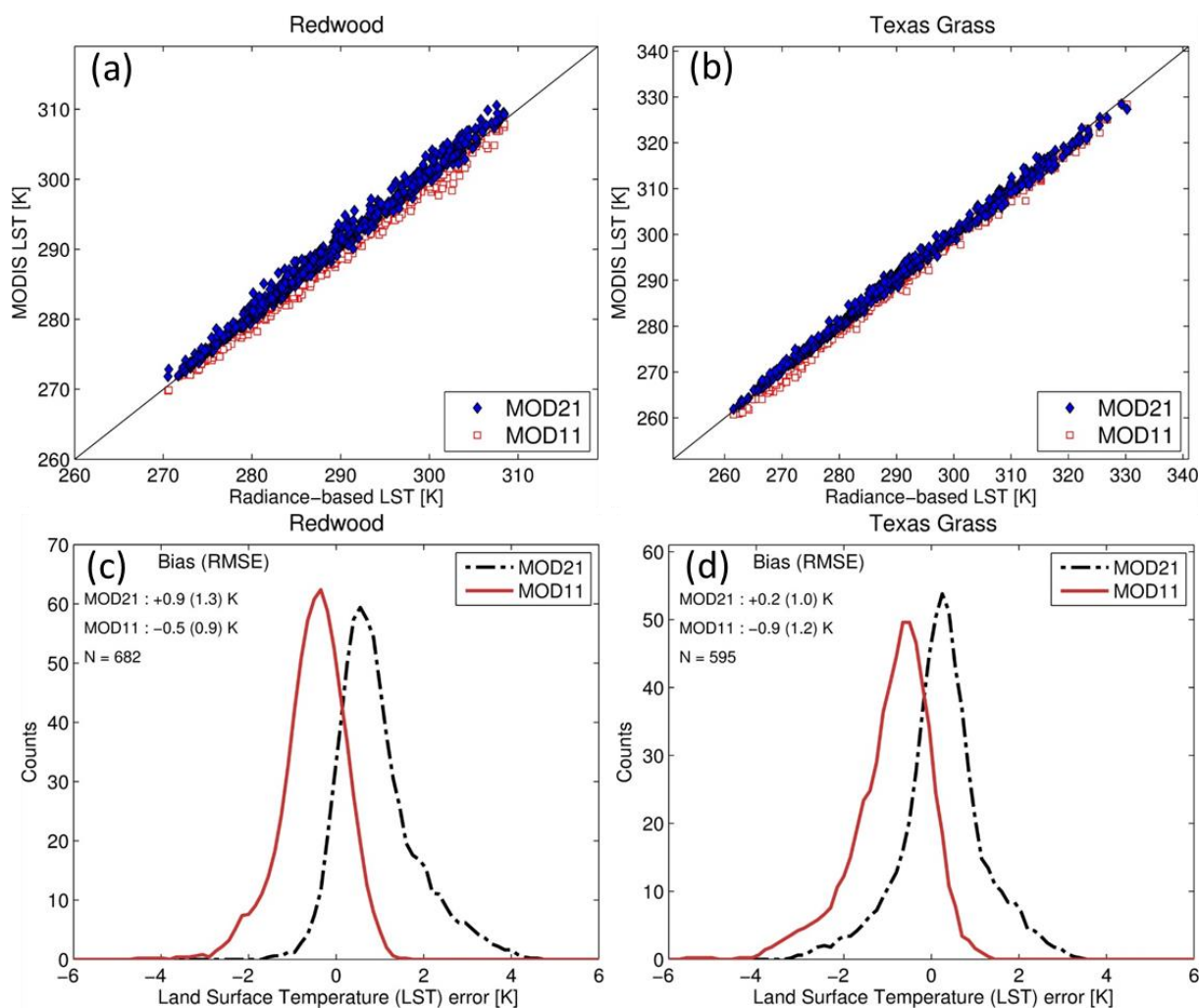
Figure 30. An example of the LST validation applied to the MODIS Aqua MOD11 and MOD21 LST products over Redwood and Texas Grassland sites (a, b) using three years of data collected (2003-2005). The bottom panels (c,d) show the histogram of the distribution of the LST error for MOD21 and MOD11 showing comparable performances.
